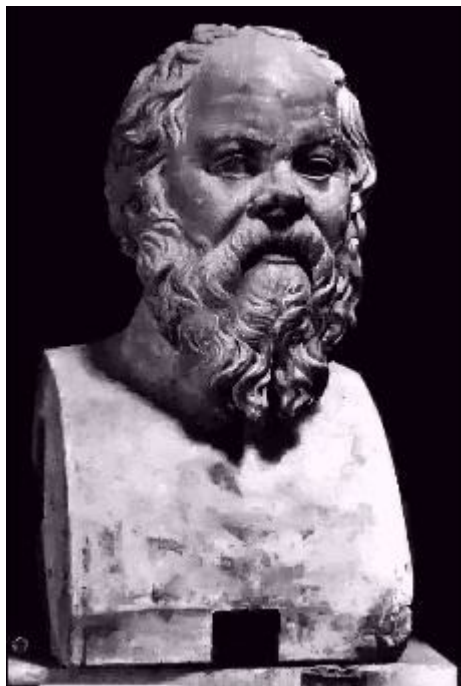
Figure 35: Socrates.
