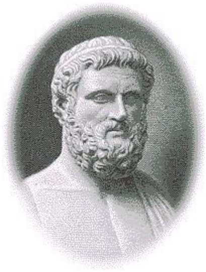
Figure 30: Solon.
