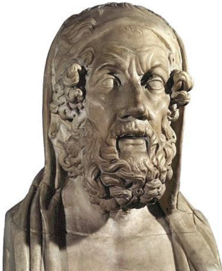
Figure 34: Homer.
